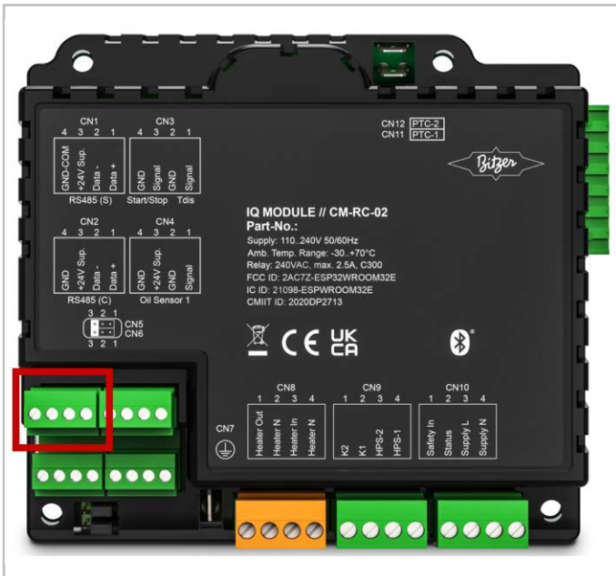
Fig. 8: Modbus connector for the communication with the gateway on IQ MODULE CM-RC-02
