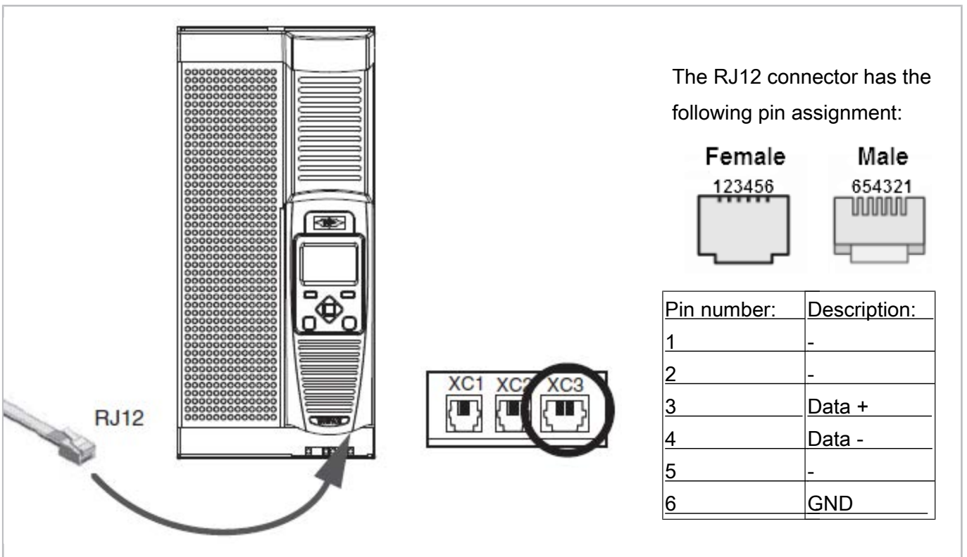
Fig. 13: Terminals of the Modbus interface socket of the VARIPACK
