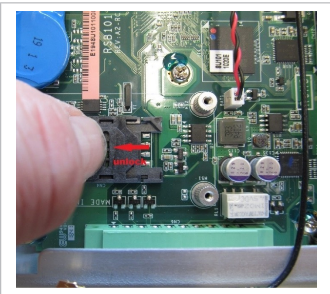
Fig. 21: Unlock the SIM card holder.
