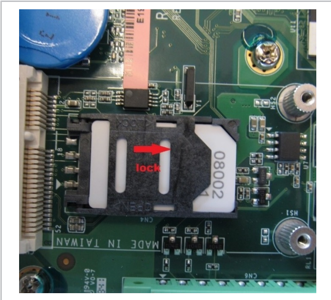
Fig. 22: Plug in the SIM card, lock the holder.
