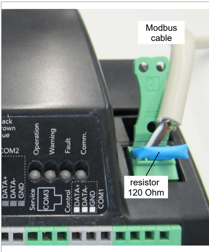
Fig. 10: Modbus connection on SE-i1
