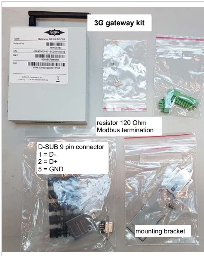
Fig. 2: Gateway kit (part no. 347 992 01) for installation in switch cabinet
