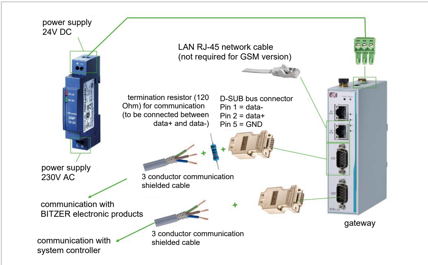
Fig. 26: Connection of the gateway in a bridge configuration
