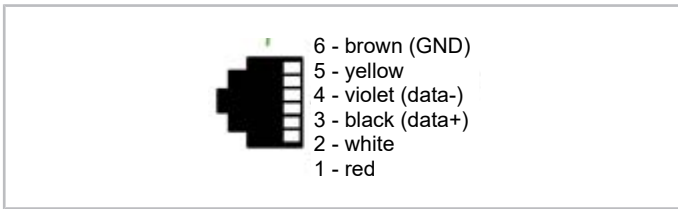
Fig. 12: RJ12 connector of pins for BEST connection on CSV and SE-i1
