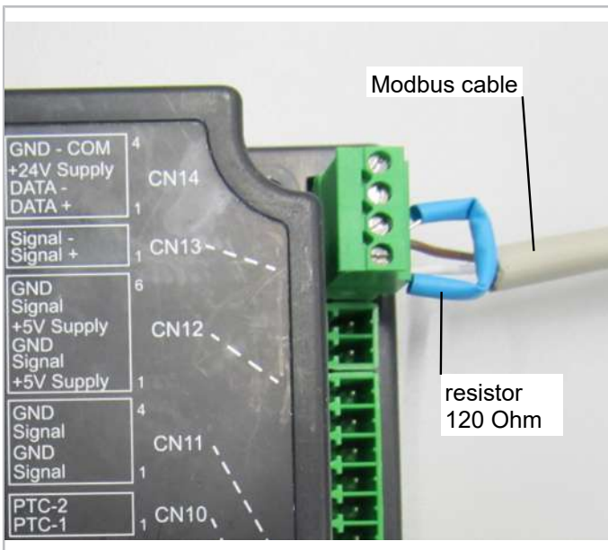
Fig. 9: Modbus /BEST connection on CM-SW-01 or CM-RC-01 (both protocols are possible at the same connection)
