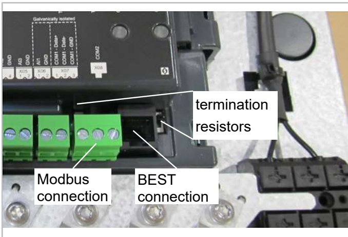
Fig. 11: Modbus/BEST connection at CSV compressor
