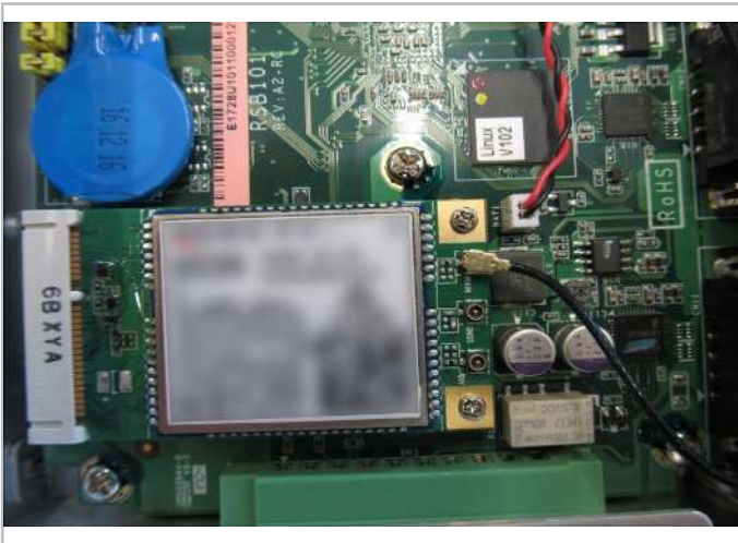
Fig. 23: Reinstall the GSM module and plug in the antenna cable.
