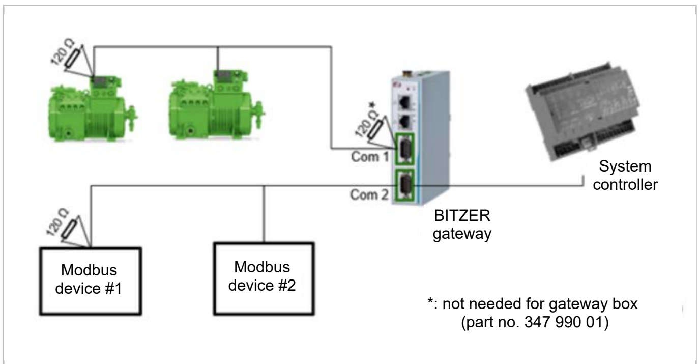
Fig. 25: Bridge configuration: general setup
