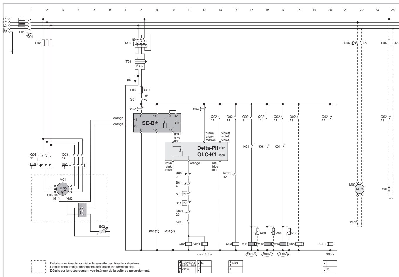
Fig. 8: 6-cylinder compressor with protection device SE-B* and part winding start, CR11 maximum equipment
