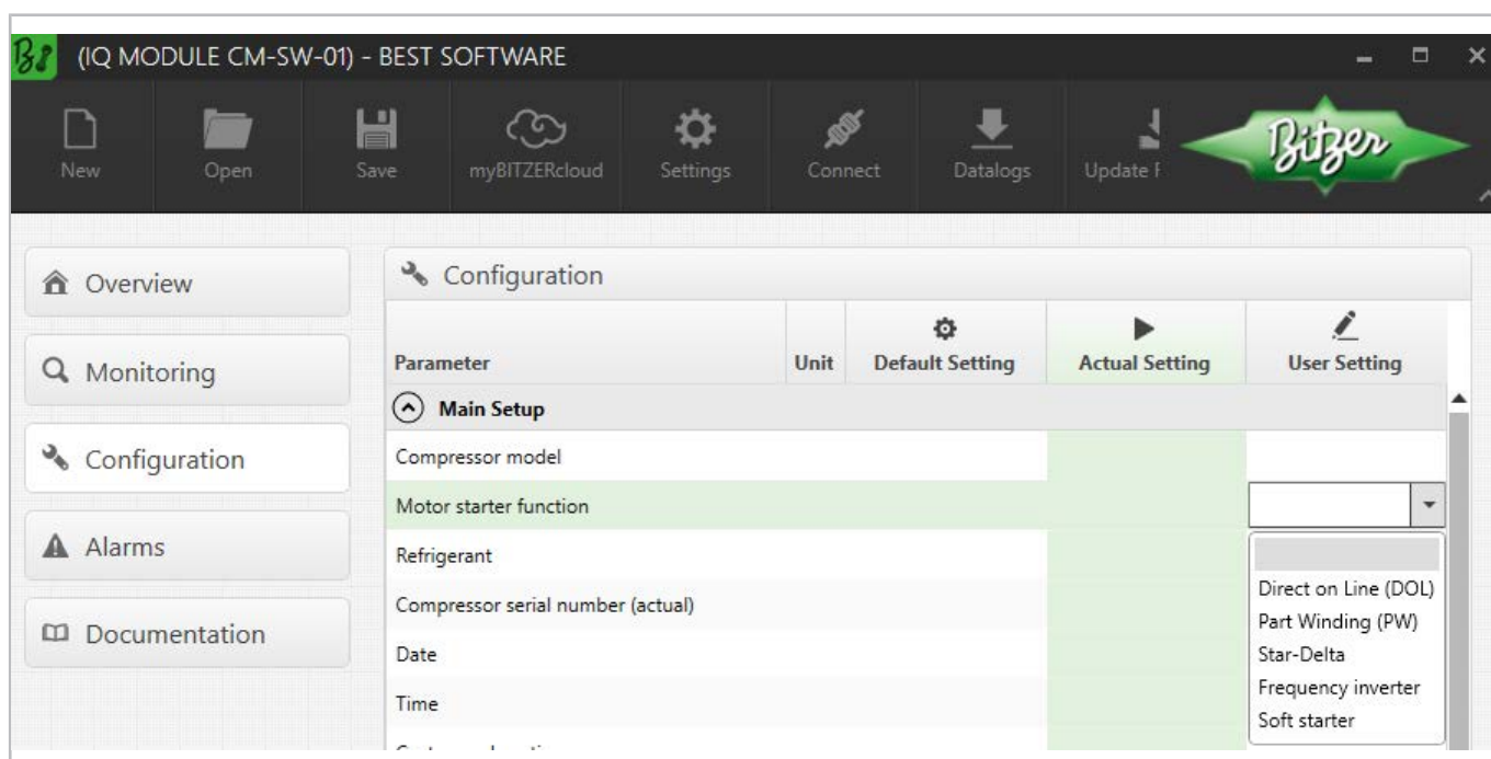
Fig. 15: Choosing the starting mode in the BEST SOFTWARE, here with CM-SW-01.
