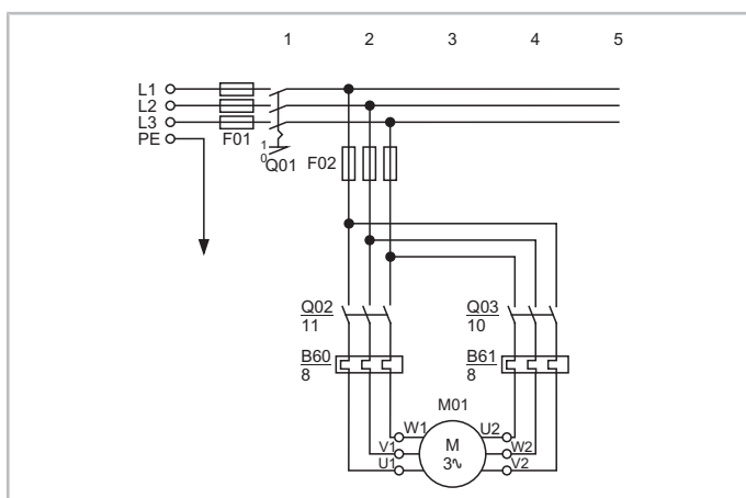
Fig. 39: Part winding start for an OS.85 screw compressor Q02: contactor for 1. part winding Q03: contactor for 2. part winding M01: motor
