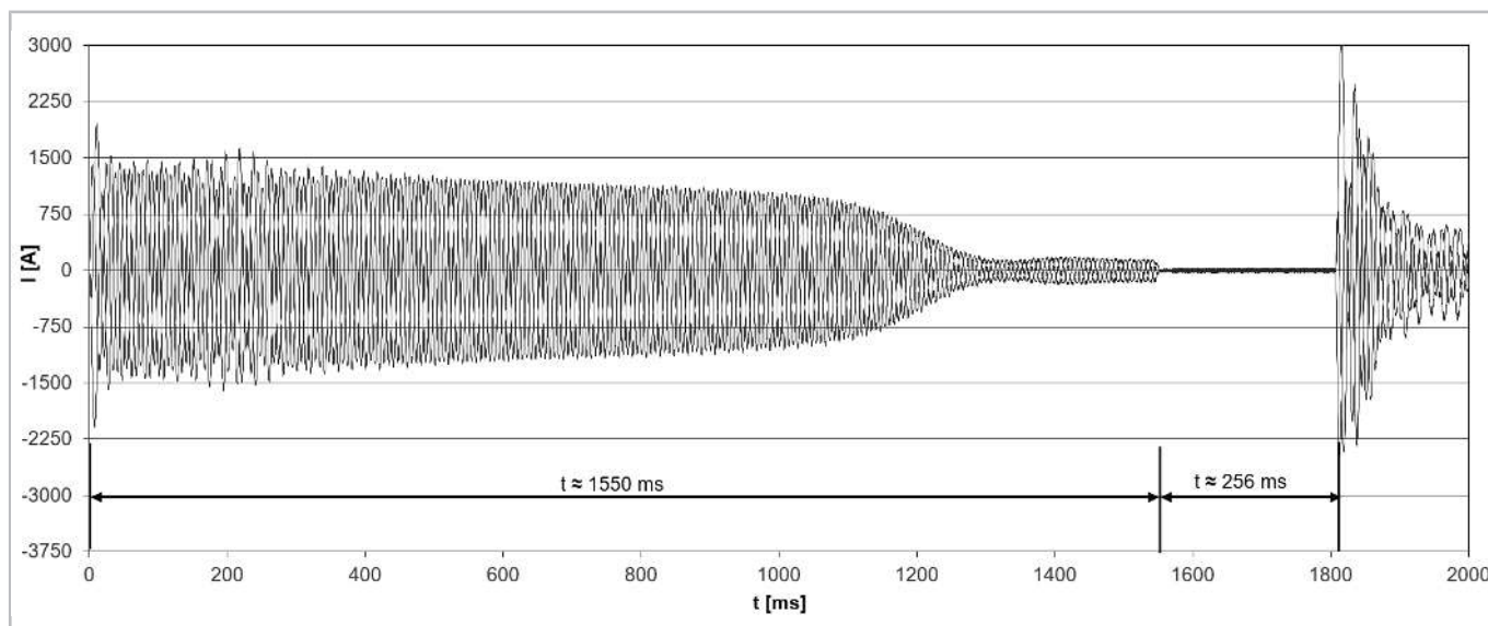
Fig. 14: Starting current (peak value) for a screw compressor model CSW10593-360Y with star-delta start. The starting current (Rotor locked) is 955 A (star) / 2913 A (delta).
