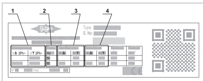
Fig. 21: Compressor with a direct-on-line start motor, example of a name plate
