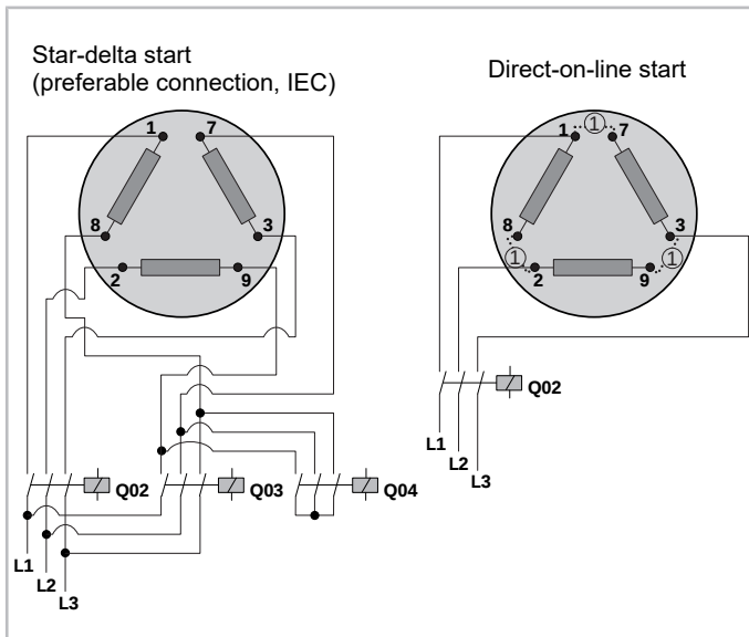
Fig. 28: Schematic illustration of the internal wiring in the motor for star-delta start Q02: main contactor (star-delta start) resp. compressor contactor (direct-on-line start) Q03: delta contactor Q04: star contactor (1): bridges for direct-on-line start (optional accessories)
