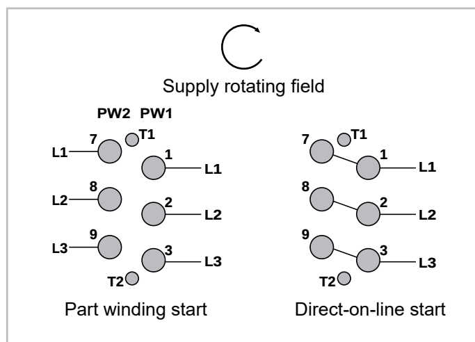
Fig. 36: Motor connection for part winding start CS.85 compressor (example)
