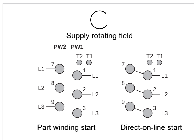
Fig. 37: Motor connection for part winding start for HS.85 compressor (example)
