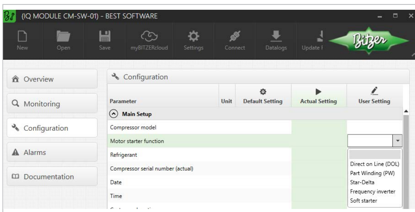
Fig. 5: Choosing the starting mode in the BEST SOFTWARE, here with CM-SW-01.
