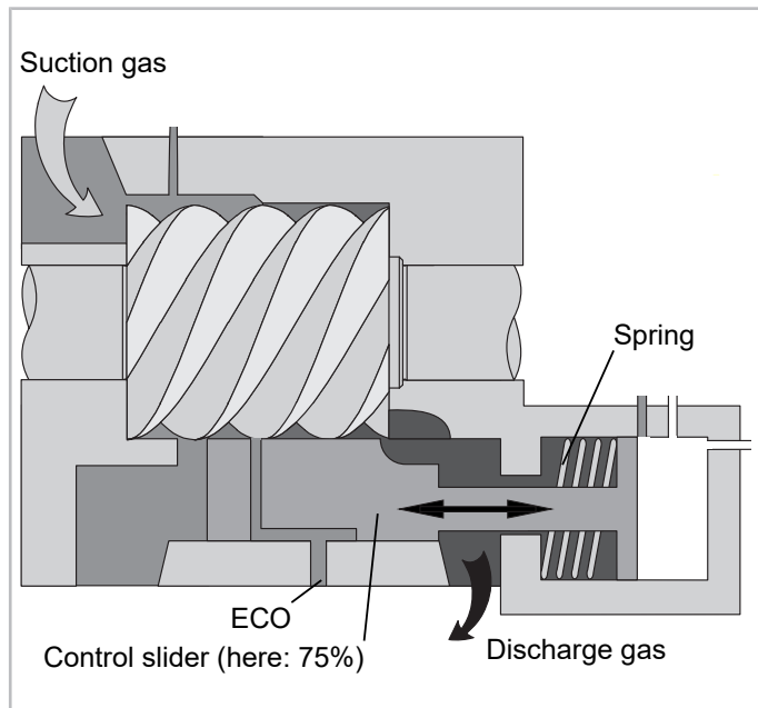
Fig. 44: Principle of slider control e.g. for a BITZER CS. screw compressor
