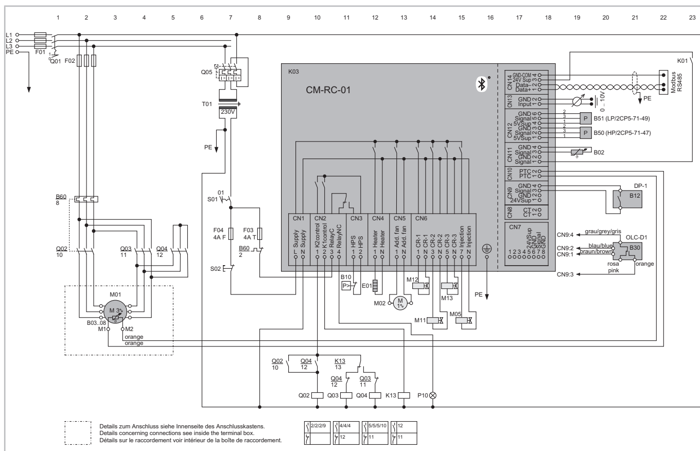
Fig. 43: ECOLINE reciprocating compressor with compressor module CM-RC-01, star-delta start and start unloading. The diagram shows the maximum possible equipment of a 6-cylinder compressor with start unloading (solenoid valve M11) and 2x CR11 capacity control (solenoid valves M12 and M13), placed here under the compressor module CM-RC-01.
