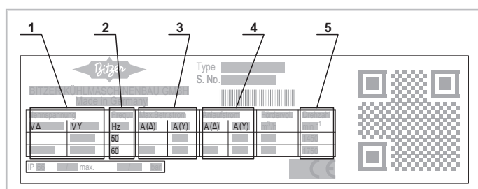
Fig. 2: Typical name plate for a built-in direct-on-line start motor that can be operated in star or delta configuration.
