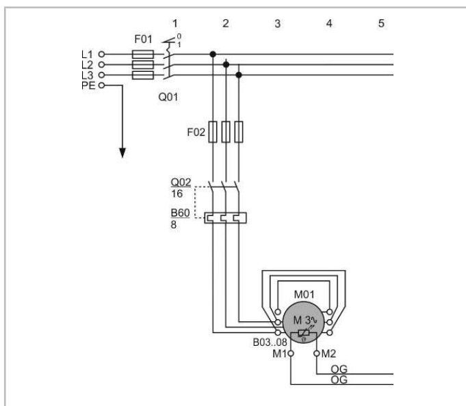
Fig. 20: Direct-on-line start in delta wiring for a reciprocating compressor
