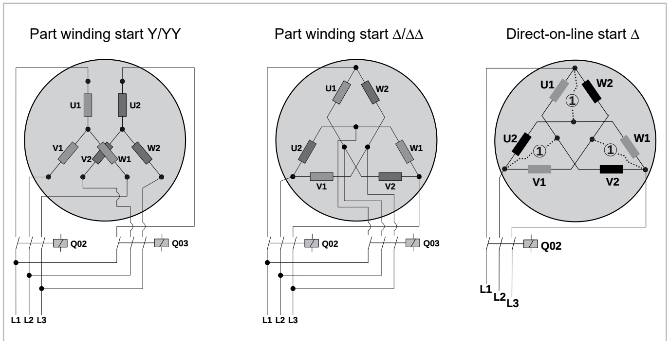
Fig. 38: Schematic illustration of the internal wiring in the motor for part winding start Q02: contactor for 1. part winding (PW1) resp. compressor contactor (direct-on-line start) Q03: contactor for 2. part winding (PW2) (1): bridges for direct-on-line start (optional accessories)
