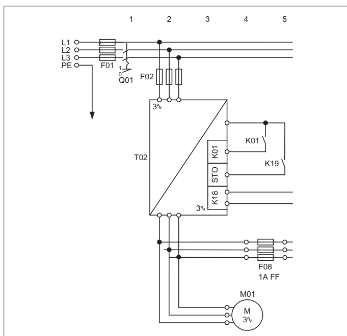
Fig. 8: Start with frequency inverter for an OS.95 screw compressor
