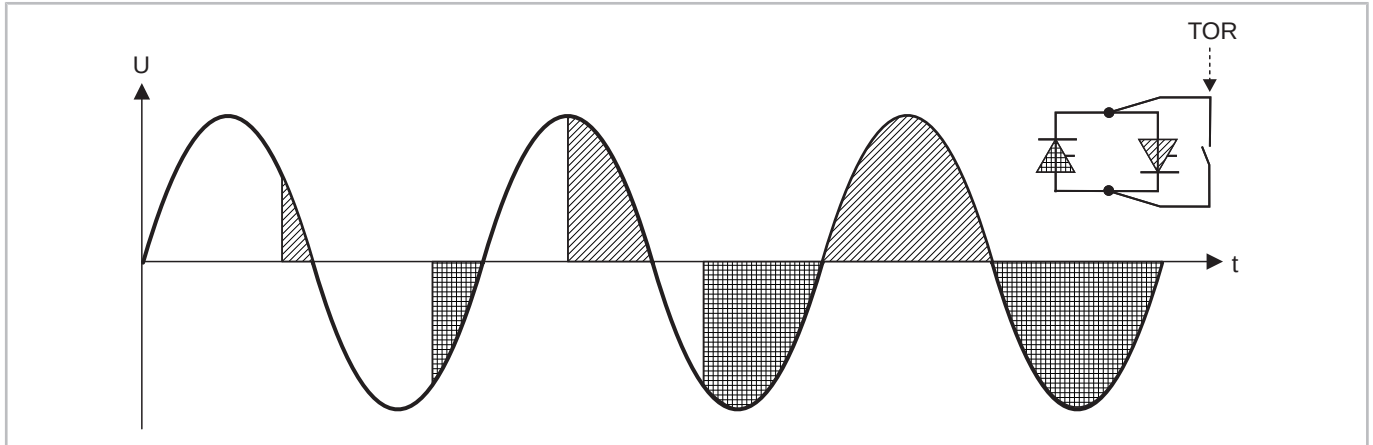
Fig. 9: Soft starter: phase angle control and bypass contact (TOR: top of ramp, full sine half-waves).
