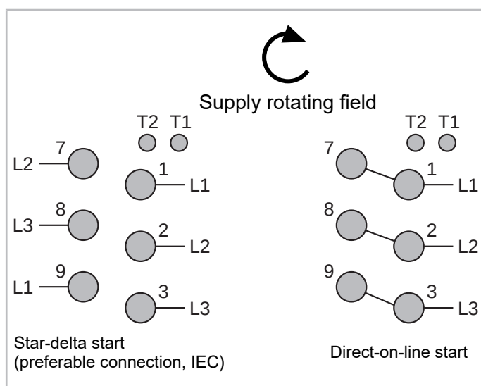
Fig. 27: Motor connection for star-delta start HS.85 compressor (example)
