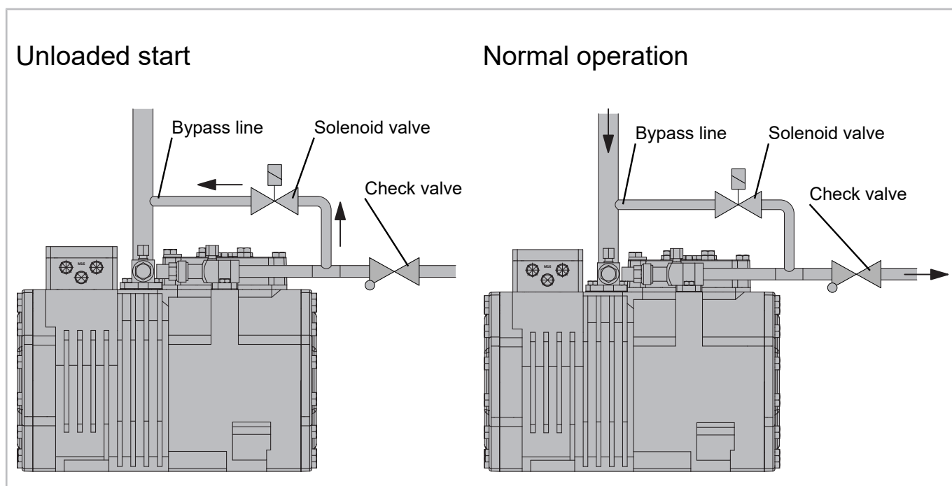
Fig. 41: External start unloading for BITZER reciprocating compressors (example)
