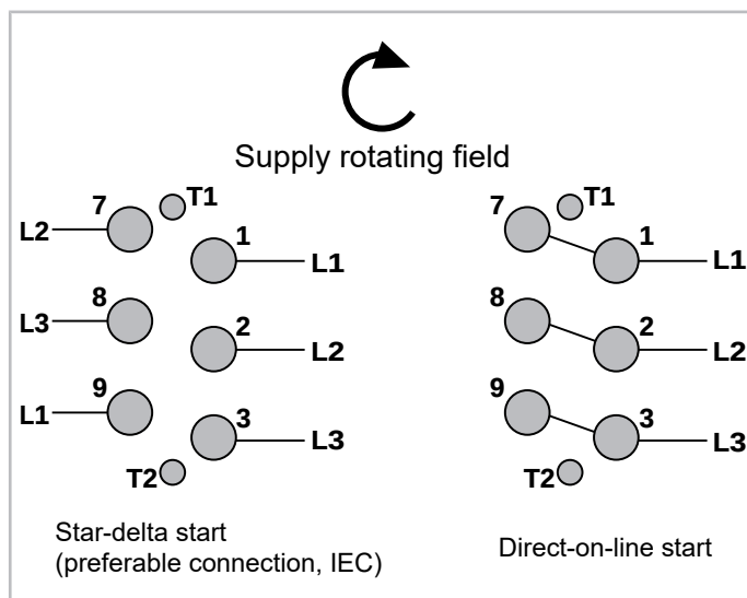
Fig. 26: Motor connection for star-delta start CS. compressor (example)
