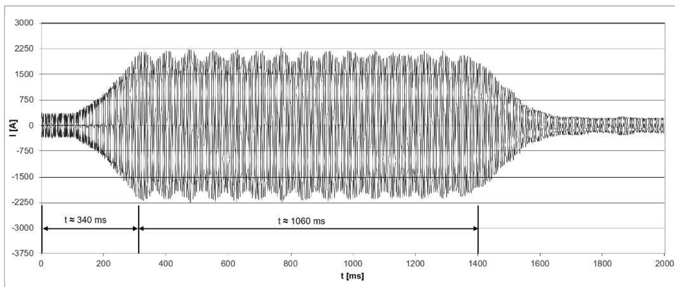
Fig. 13: Starting current (peak value) for a screw compressor model CSW10593-360Y with soft starter. Its max. operating current is 565 A.
