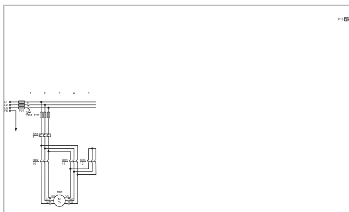
Fig. 29: Star-delta start for an OS.85 screw compressor
