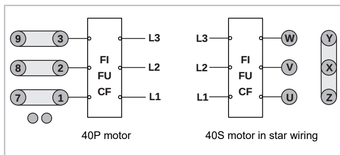
Fig. 6: Motor terminals at the terminal plate for operation with external frequency inverter (FI), examples for reciprocating compressors
