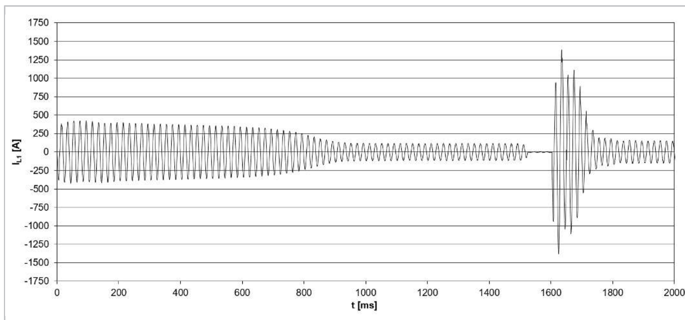
Fig. 49: Starting current (peak value) for a compressor model CSH8593-140Y with star-delta start (IEC connection) and start unloading (i.e. slider position at 75%).
