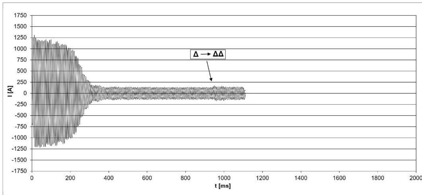
Fig. 32: Starting current (peak value) for a compressor model CSH8593-180Y with part winding start (winding partition 50% / 50%, winding type \Delta/\Delta\Delta ) and start unloading (i.e. slider position at 25% ).
