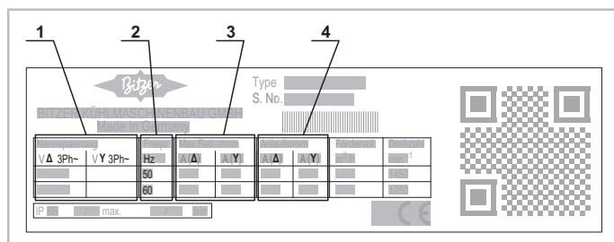
Fig. 30: Compressor with star-delta motor, example of a name plate
