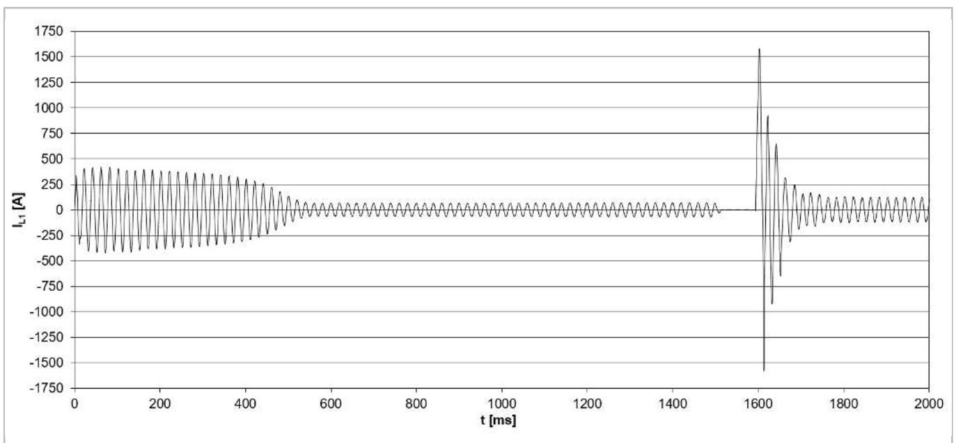
Fig. 48: Starting current (peak value) for a compressor model CSH8593-140Y with star-delta start (IEC connection) and start unloading (i.e. slider position at 50%).
