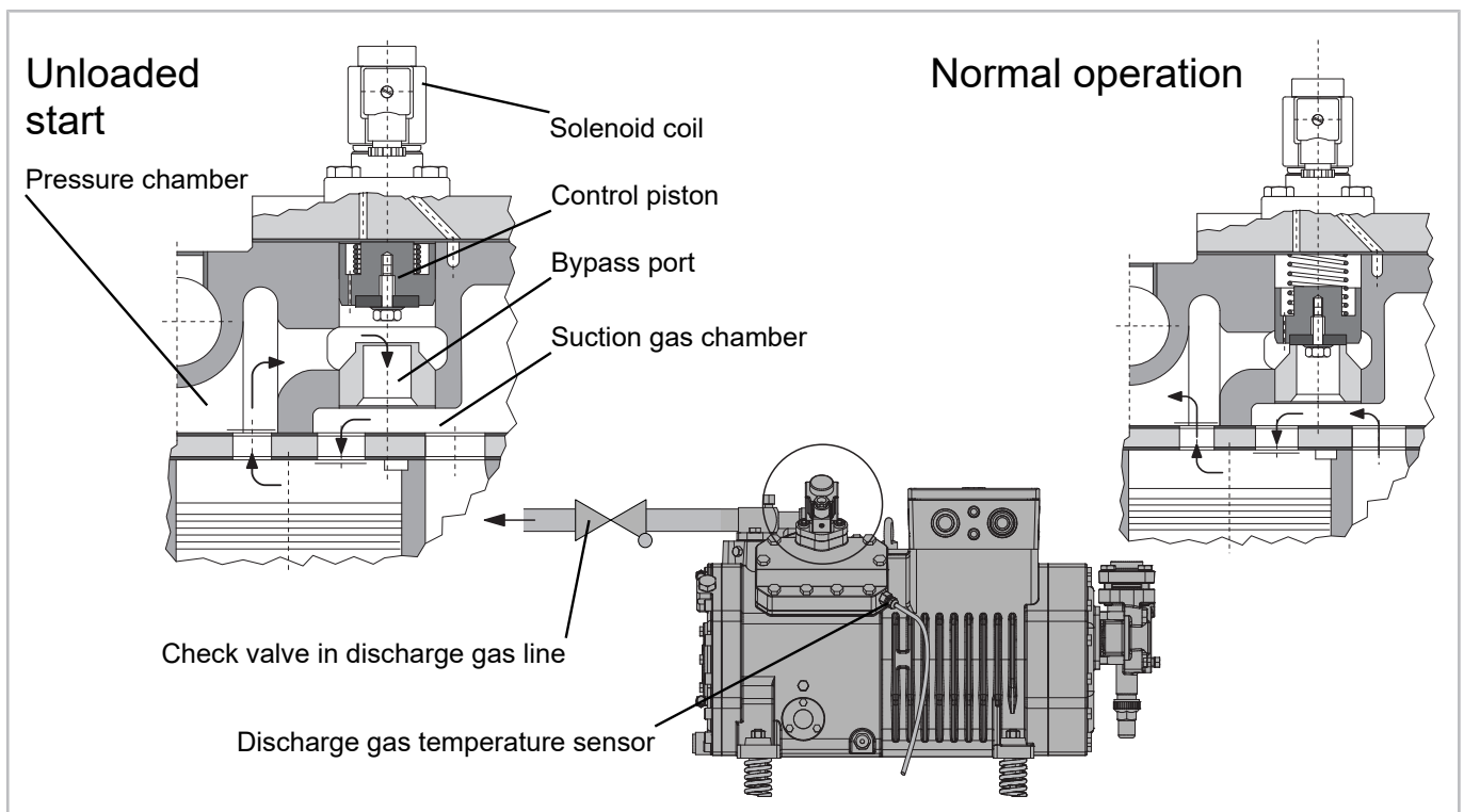
Fig. 40: Integrated start unloading for BITZER reciprocating compressors (example)
