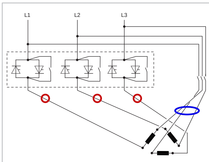
Fig. 12: Recommended connection of the rotation direction monitoring to the 3-phase controlled soft starter with inside delta connection: either at the points of the red circles or the blue ellipse.
