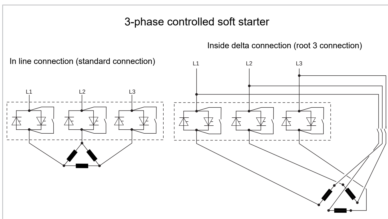
Fig. 11: Comparison of in line vs. inside delta connection of a 3-phase controlled soft starter
