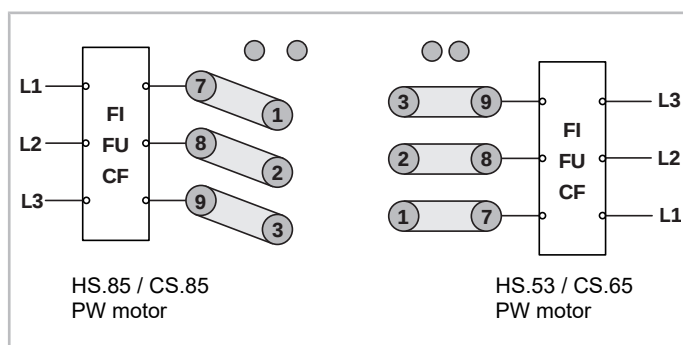
Fig. 7: Motor terminals at the terminal plate for operation with external frequency inverter (FI), examples for screw compressors
