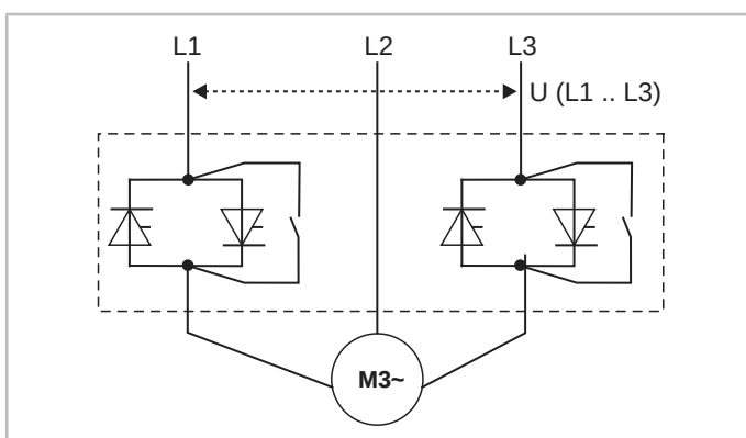
Fig. 10: Schematic structure of a 2-phase controlled soft starter with integrated bypass contacts
