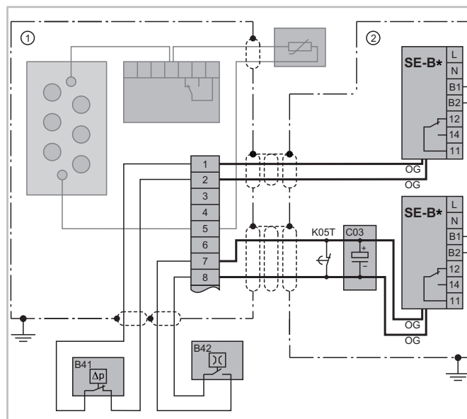
Fig. 39: Electrical connection of integrated oil management system with terminal box ① and switch cabinet ②
