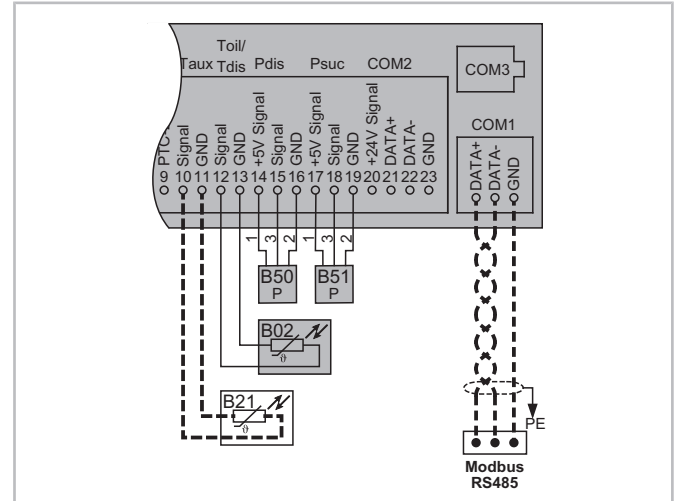
Fig. 36: SE-i1 on HS., part 2: The three sensors: High and low pressure transmitter (B50, B51) and discharge gas temperature sensor (B02) are mounted on the compressor and electrically connected as delivered. Modbus and an optional temperature sensor (B21) can be connected. NTC sensors must be used for both temperature sensors (B02 and B21).
