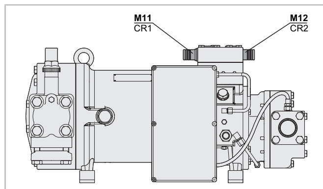
Fig. 24: HS.53: Position of the solenoid valves
