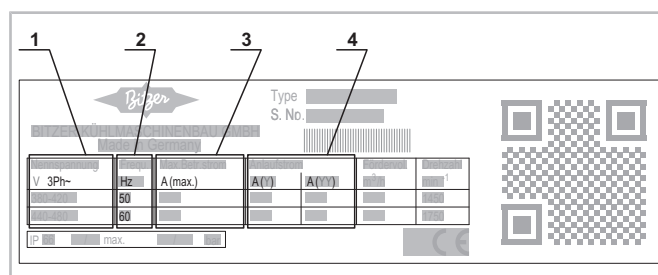
Fig. 11: Compressor with part winding motor, example of a name plate
