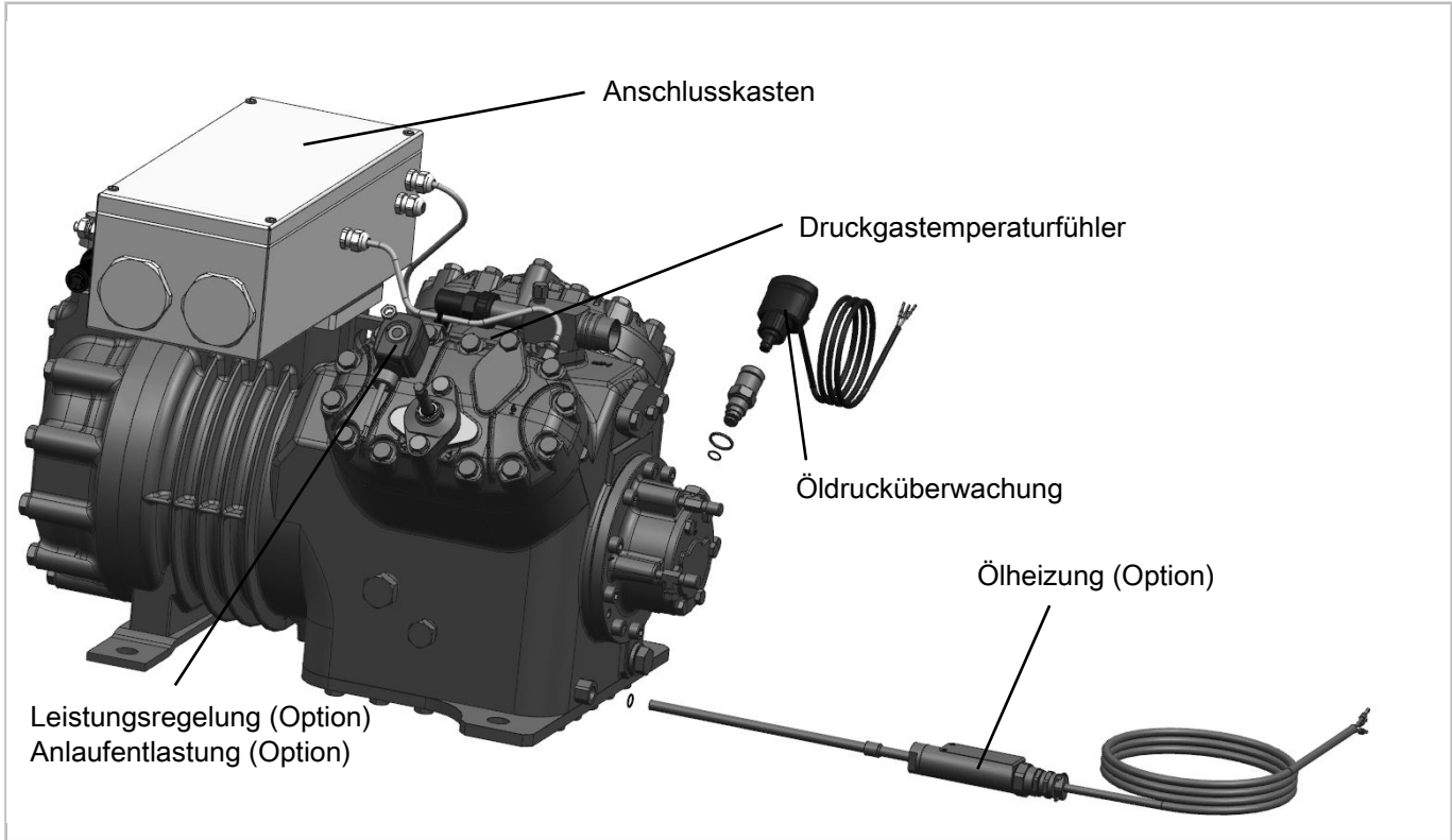
Abb. 7: 4JE(P)-13.EX(Y/P) .. 4FE(P)-35.EX(Y/P)
