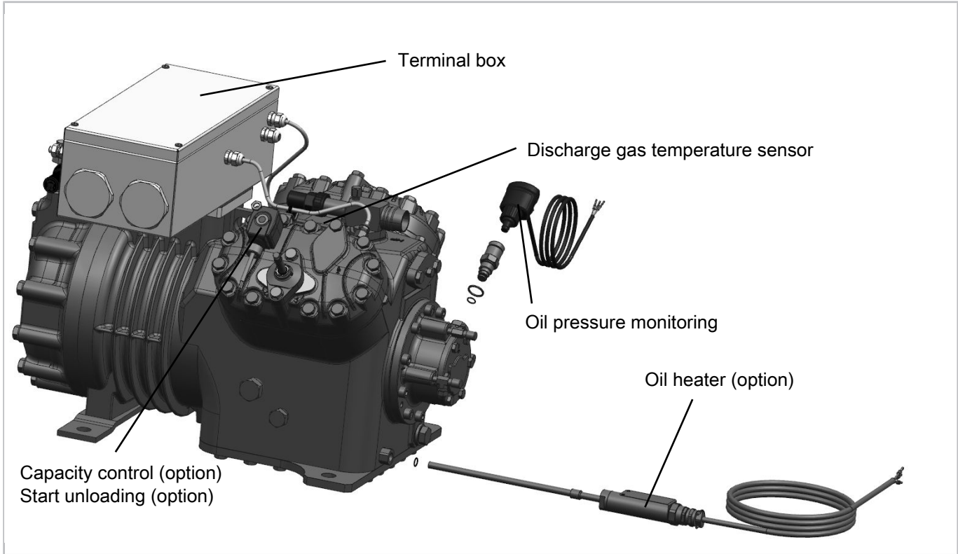
Fig. 7: 4JE(P)-13.EX(Y/P) .. 4FE(P)-35.EX(Y/P)
