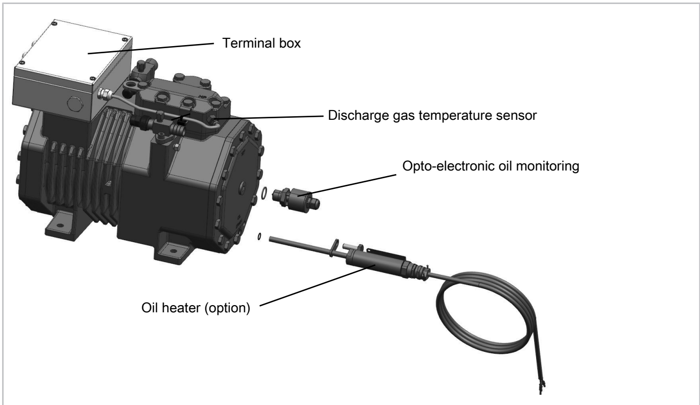
Fig. 4: 2EES(P)-2.EX(Y/P) .. 2CES(P)-4.EX(Y/P)
