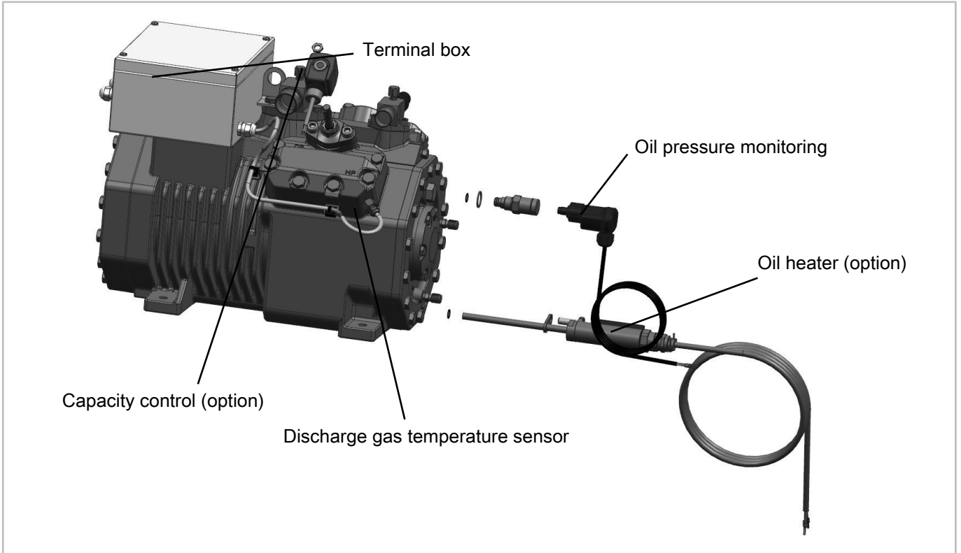
Fig. 5: 4FE(P)-3.EX(Y/P) .. 4BE(P)-9.EX(Y/P)
