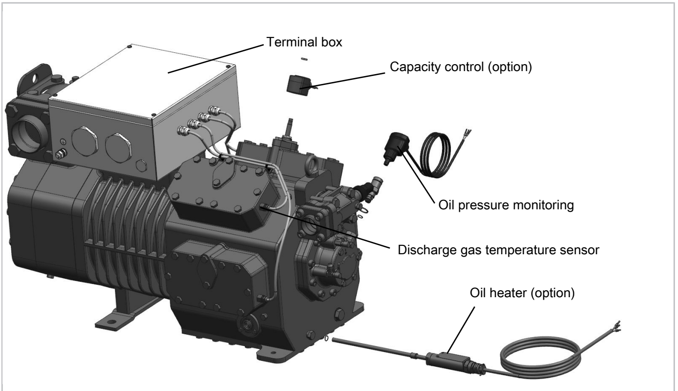
Fig. 9: 8GE(P)-50.EX(Y/P) .. 8FE(P)-70.EX(Y/P)
