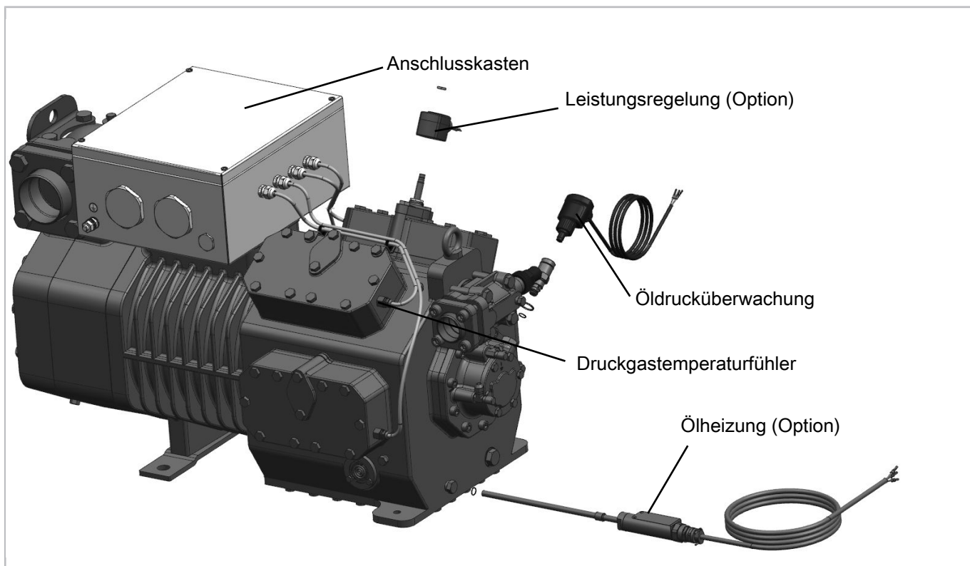
Abb. 9: 8GE(P)-50.EX(Y/P) .. 8FE(P)-70.EX(Y/P)
