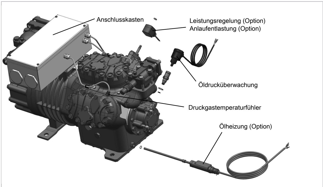
Abb. 8: 6JE(P)-22.EX(Y/P) .. 6FE(P)-50.EX(Y/P)
