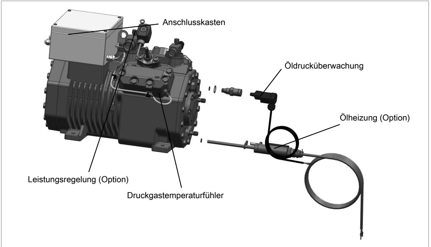
Abb. 5: 4FE(P)-3.EX(Y/P) .. 4BE(P)-9.EX(Y/P)
