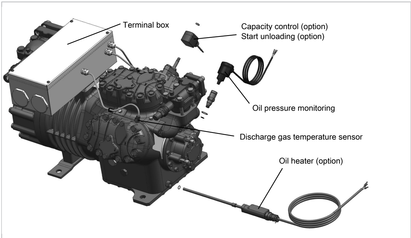
Fig. 8: 6JE(P)-22.EX(Y/P) .. 6FE(P)-50.EX(Y/P)
