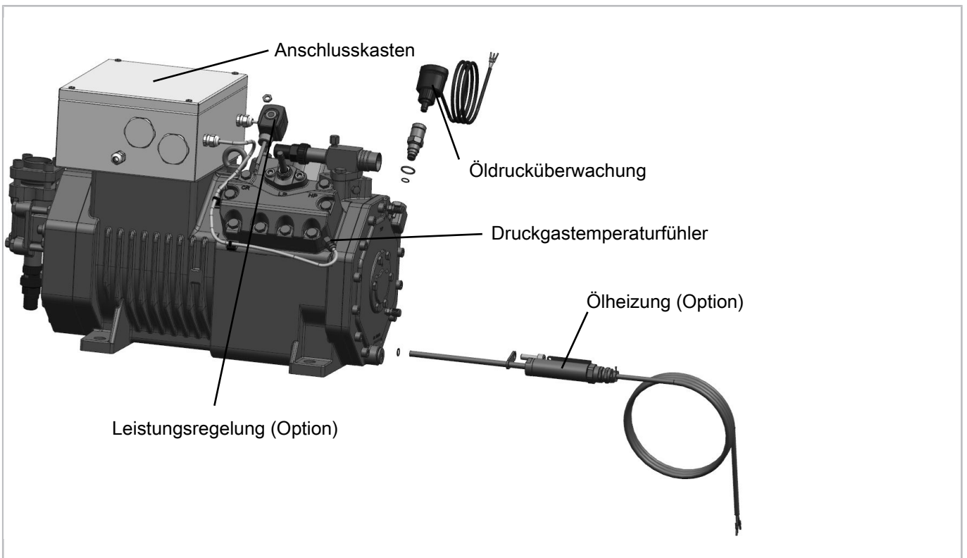
Abb. 6: 4VE(P)-6.EX(Y/P) .. 4NE(P)-20.EX(Y/P)
