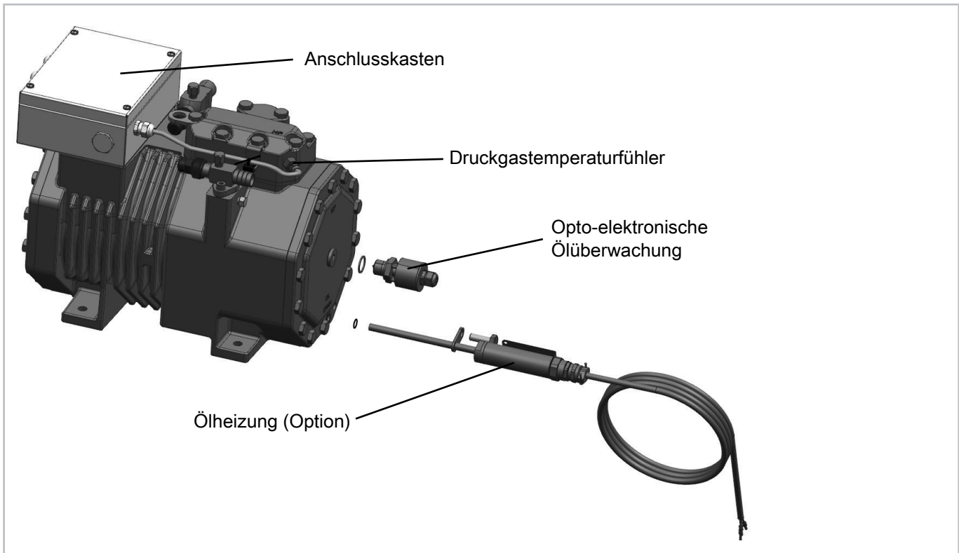
Abb. 4: 2EES(P)-2.EX(Y/P) .. 2CES(P)-4.EX(Y/P)
