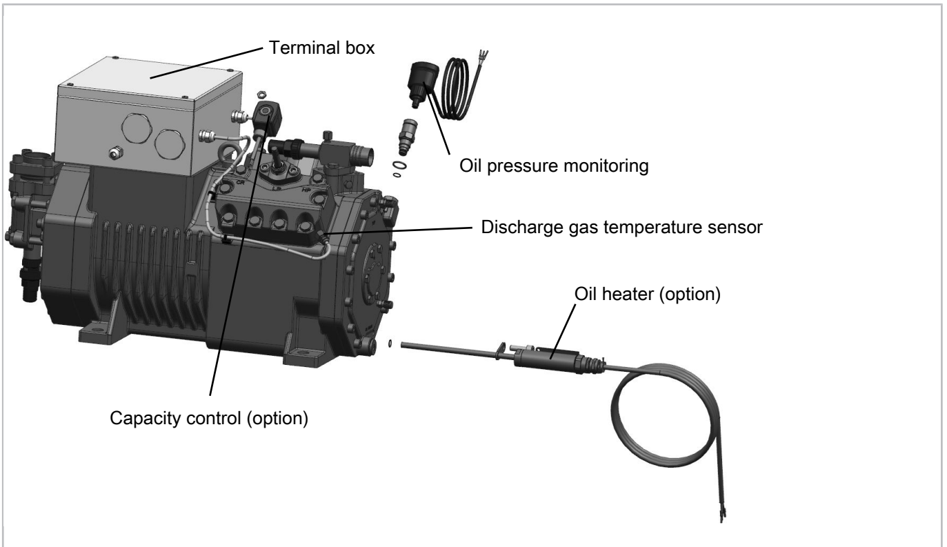
Fig. 6: 4VE(P)-6.EX(Y/P) .. 4NE(P)-20.EX(Y/P)
