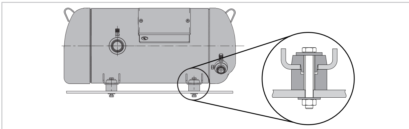
Fig. 4: Vibration damper
